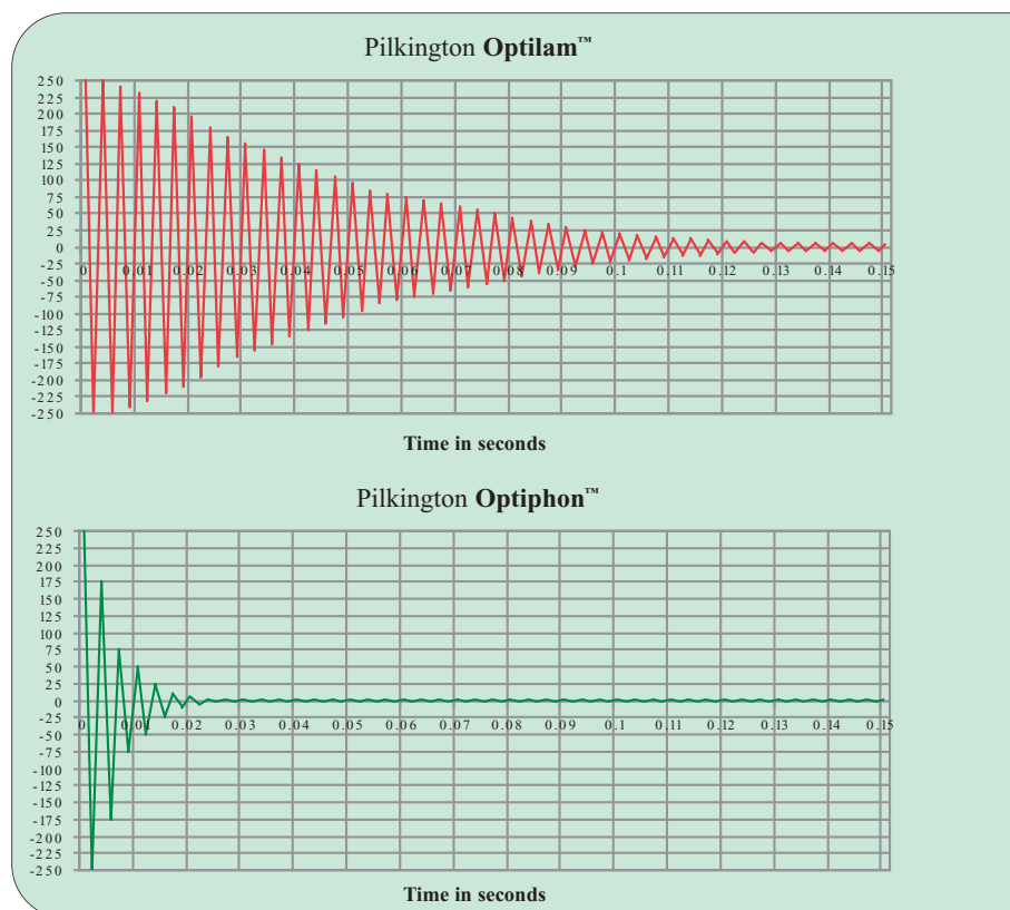
Figure 9: The illustration shows the impressive damping differences between Pilkington Optilam™ and Pilkington Optiphon™ from the sound engineering point of view.
