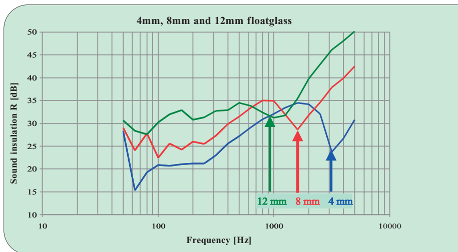
Figure 6: Influence of the pane thickness on the coincidence frequency
