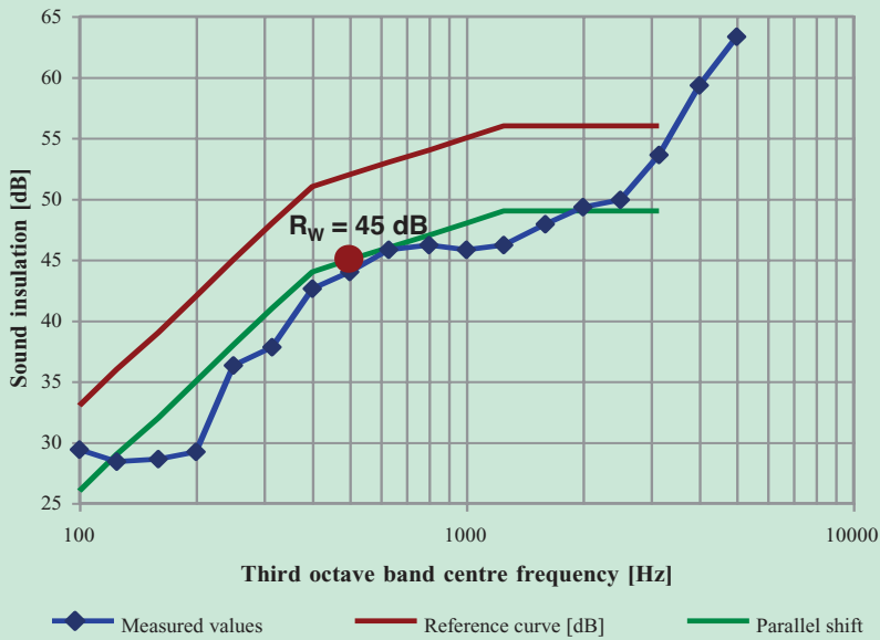
Figure 4: Determining the sound insulation
