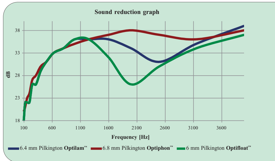
Figure 8: Sound reduction illustration
