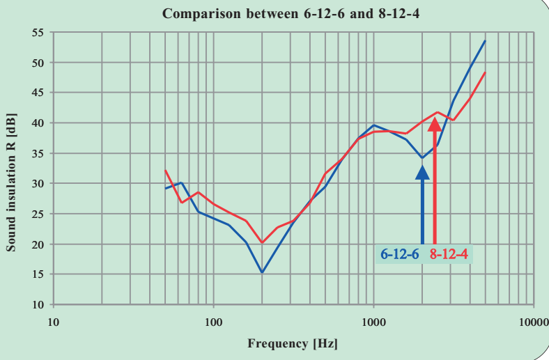
Figure 7: Asymmetric glass structure to reduce coincidence
