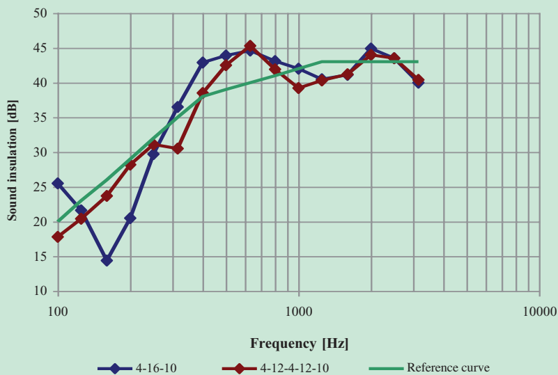
Figure 5: Comparison between two insulating glass structures
